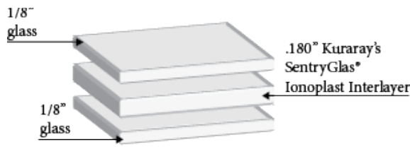
Standard monolithic Sentry Guard Construction OA thickness: 7/16" • Weight: 4.16lbs/sqft
